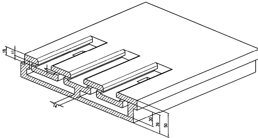
3D Replay SEC D-D SCALE 1:2
