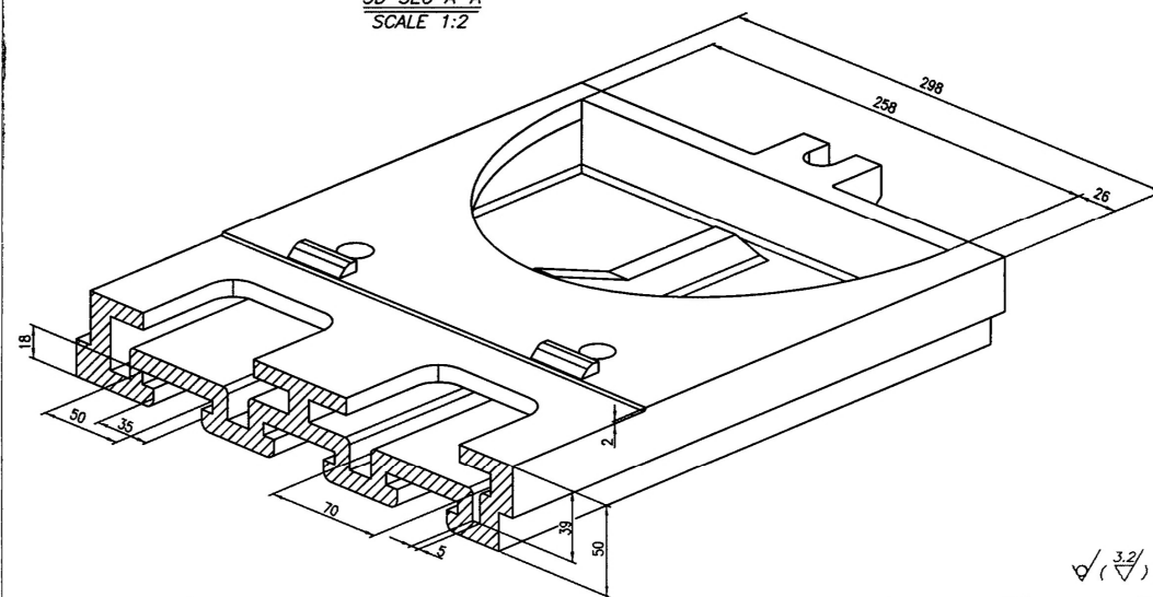
3D Replay SEC E-E SCALE 1:2
