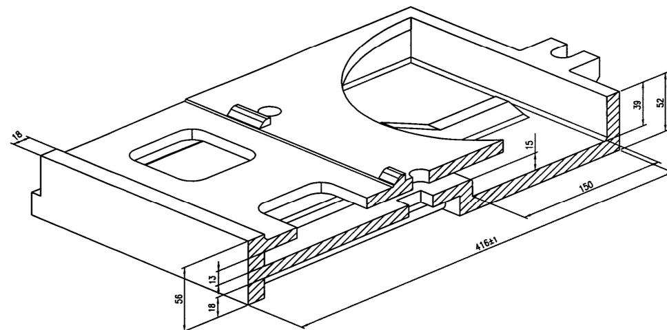
3D SEC A-A SCALE 1:2
